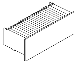
Letter, Legal, and A4 Filing 25 5/8" (657mm)
