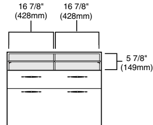
Lateral storage shelf dimensions
