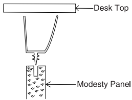
Wire Management Channel Detail
